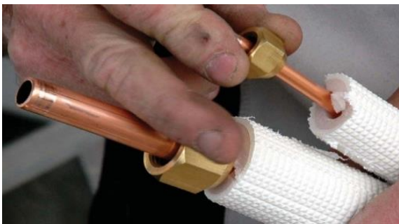
Figure 32: Flare the end of the tube (A)
