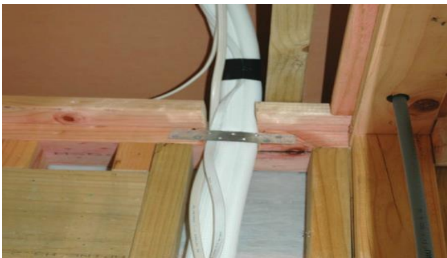
Figure 48: Fix galvanised mild steel strap to hold pipe and connection cable
