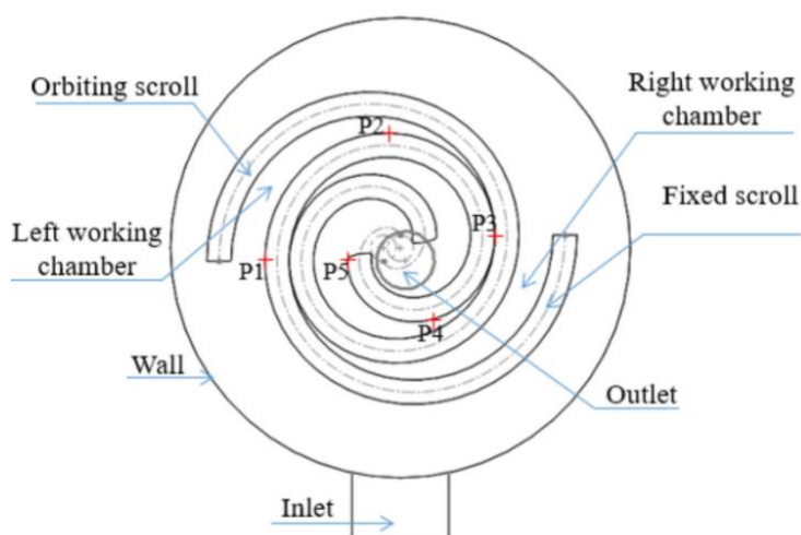
Figure 10: Scroll compressor
