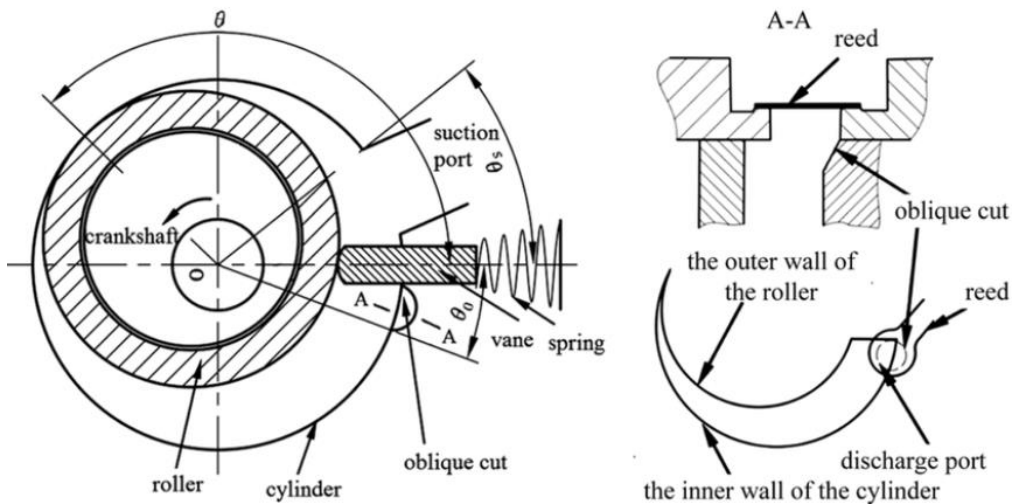
Figure 11: Rotary compressor
