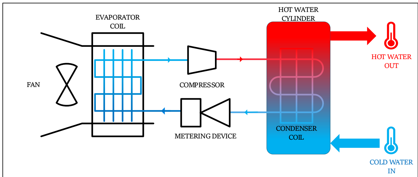
Figure 3: Air-to-water heat pump
