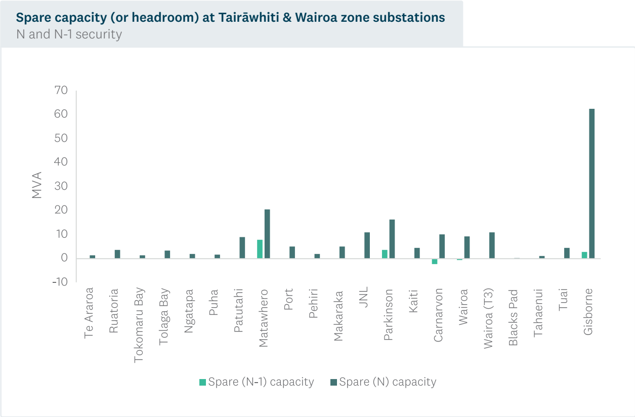
Figure 55 – Spare capacity at Firstlight Network’s Tairāwhiti and Wairoa’s zone substations. Source: ElectroNet
