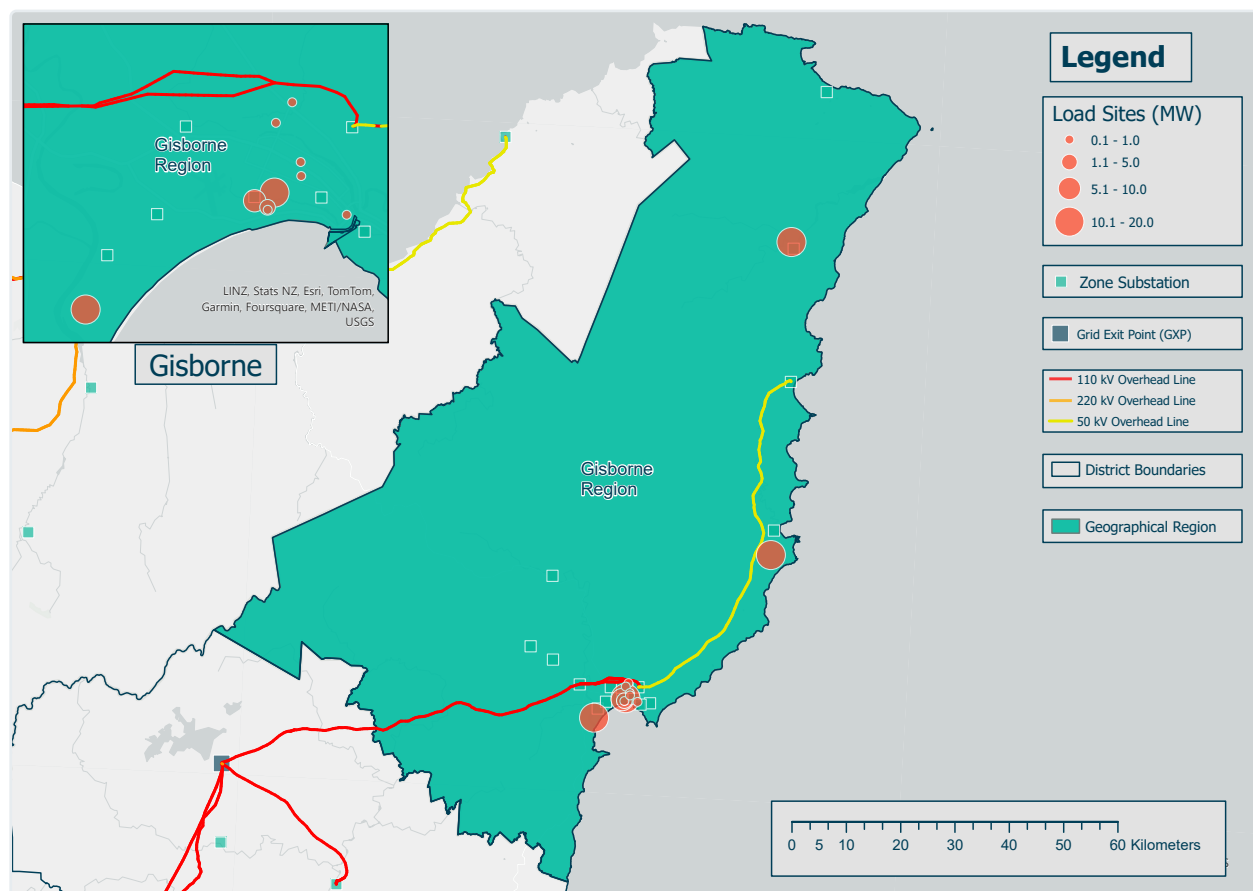
Figure 46 – Map of the Tairāwhiti and Wairoa transmission grid, location, and peak demand of RETA sites
