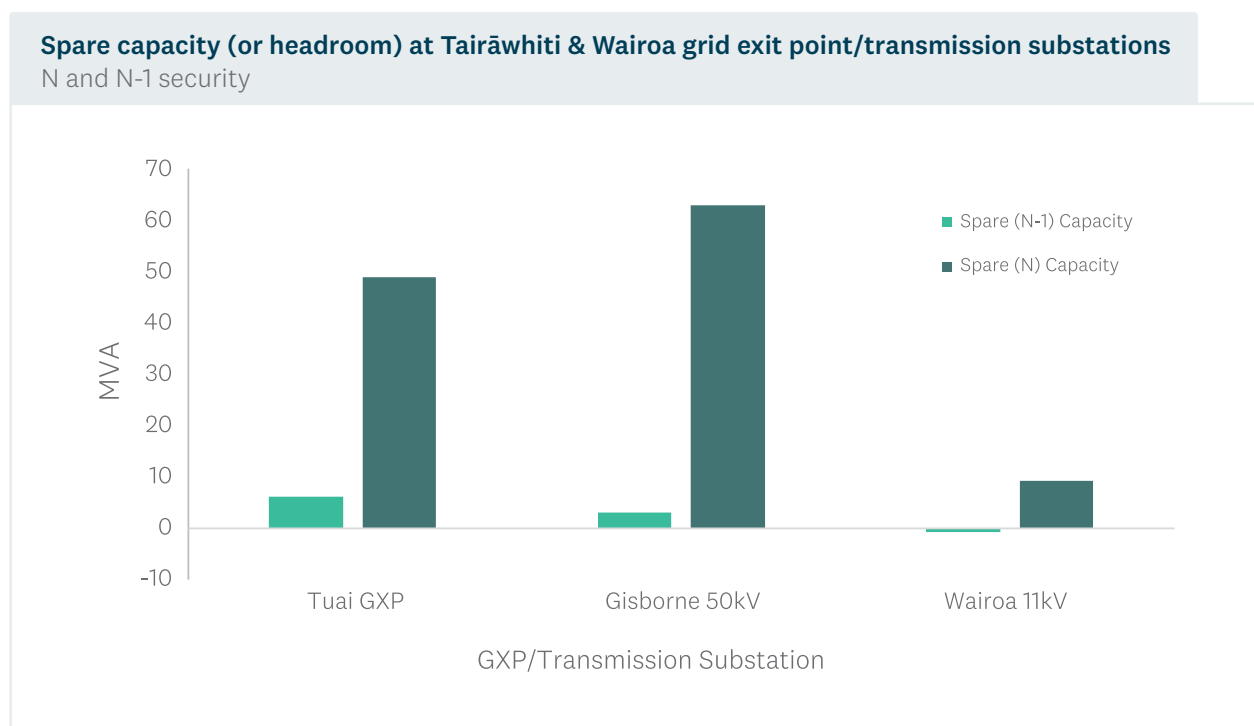
Figure 54 – Spare capacity at Transpower’s Tairāwhiti and Wairoa’s Grid Exit Points (GXP) and sub-transmission substations. Source: ElectroNet
