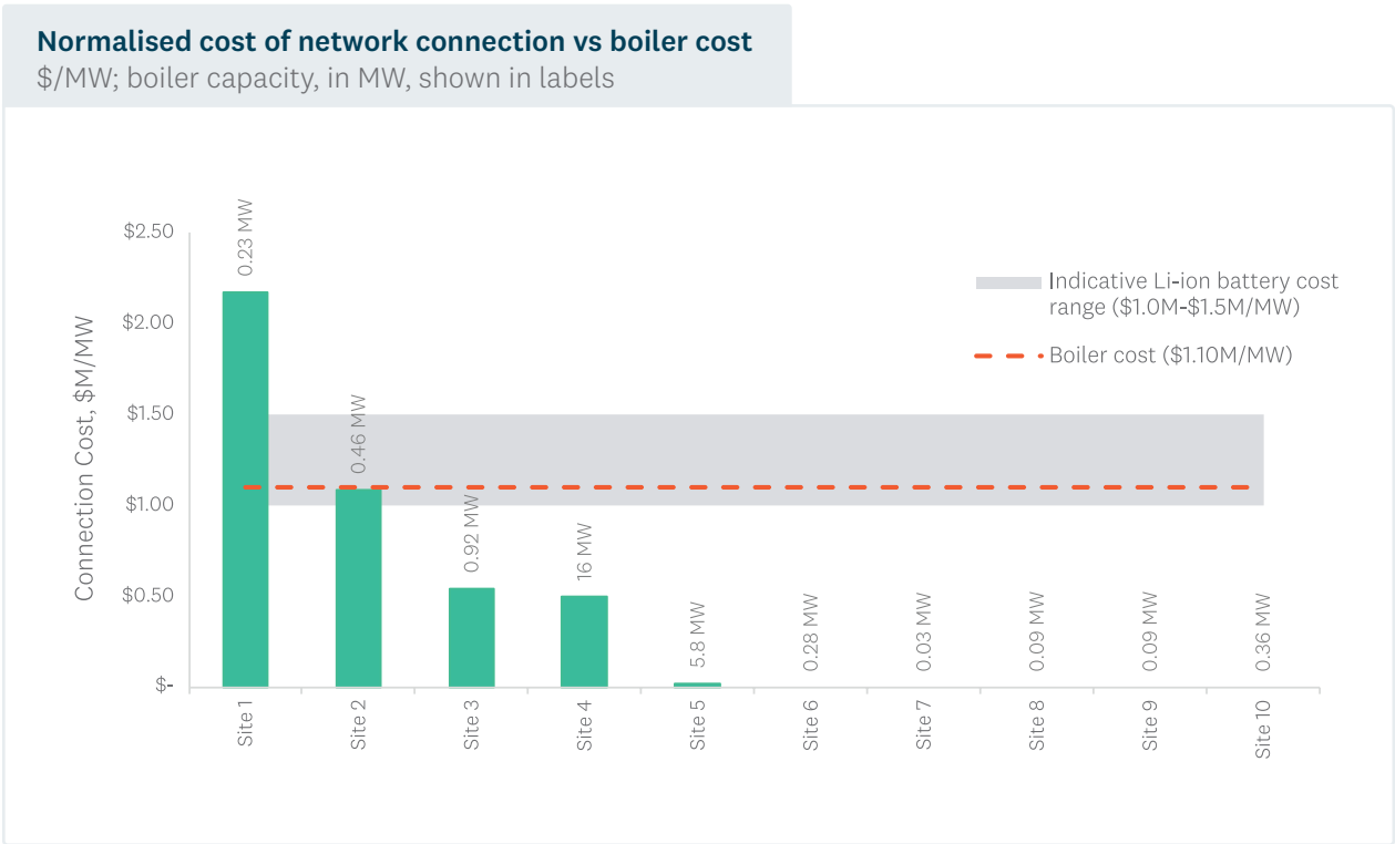
Figure 56 – Normalised cost of network connection vs boiler cost. Source: ElectroNet, EECA
