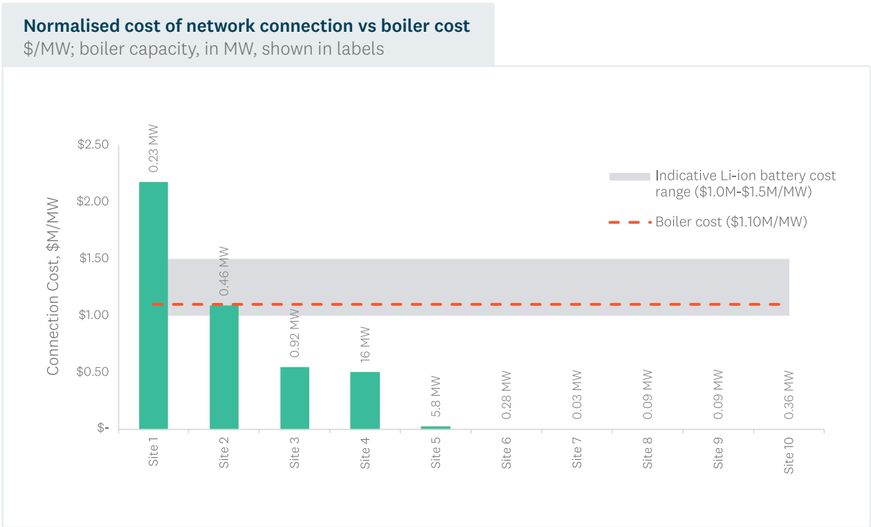
Figure 10 – Normalised cost of network connection vs boiler cost. Source: ElectroNet, EECA
