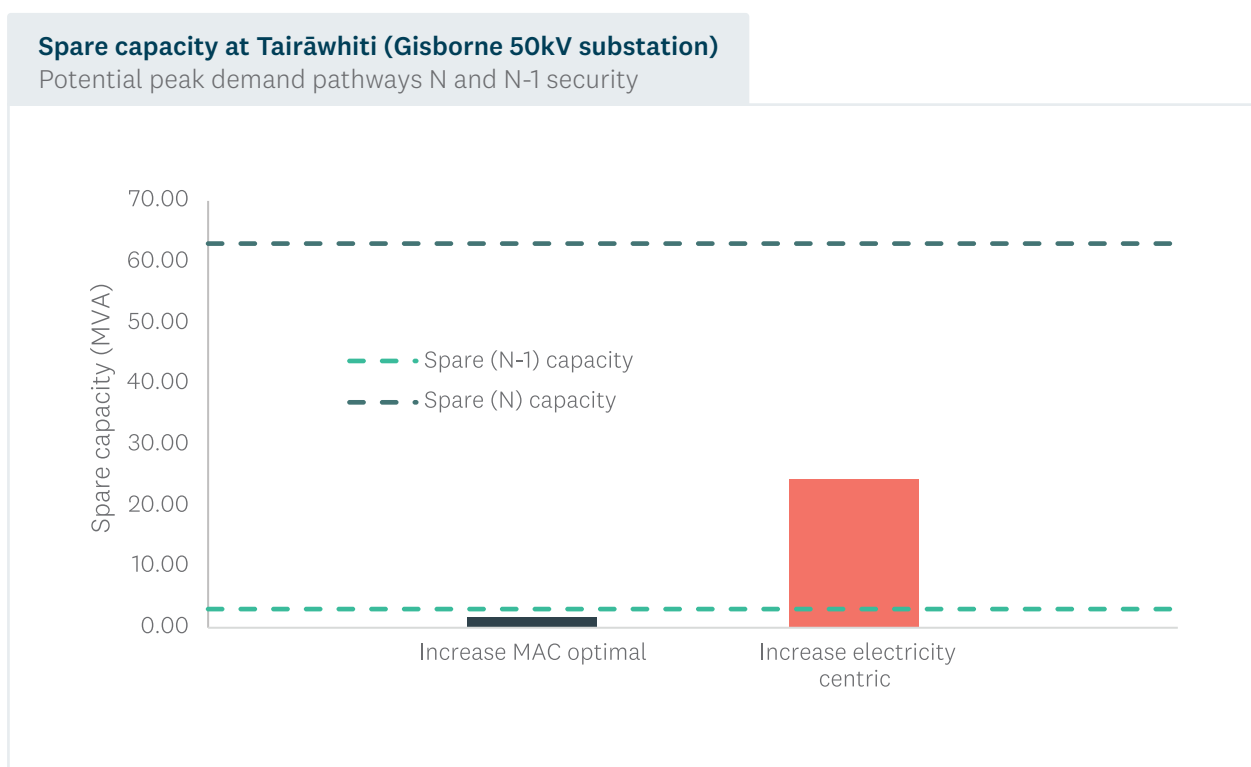
Figure 57 – Potential combined effect of site decisions at Gisborne zone substation on spare capacity. Source: ElectroNet
