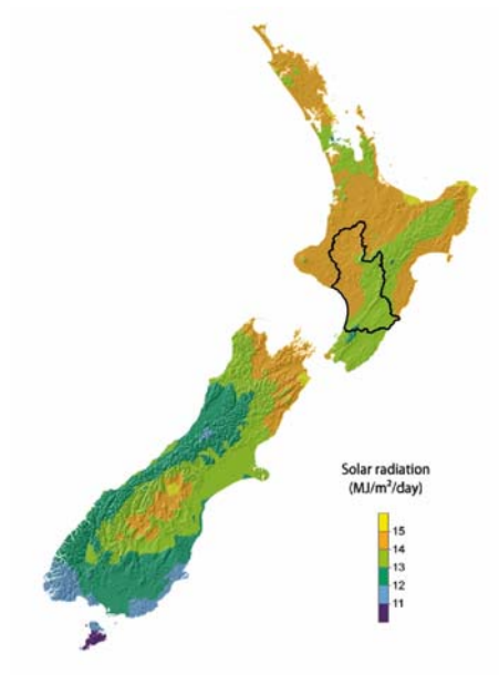
■ Figure 12 Solar radiation distribution (NIWA 2005b)
