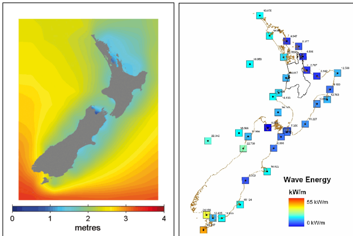
■ Figure 20 Mean wave height from 1979 to 1998 and wave energy (NIWA 2006d, East Harbour Management Services 2005)
