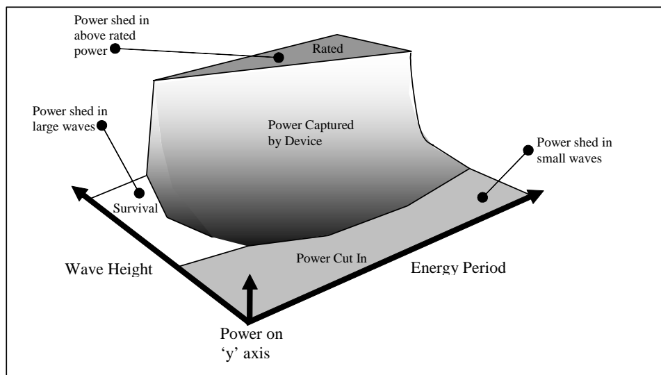
■ Figure 19 Typical wave device power capture
