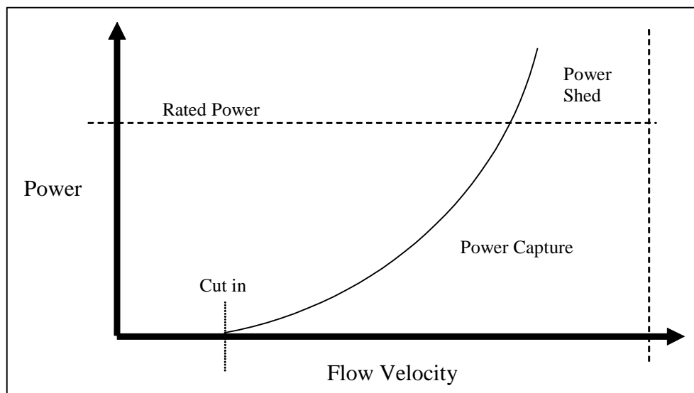
■ Figure 18 Generic device power capture graph
