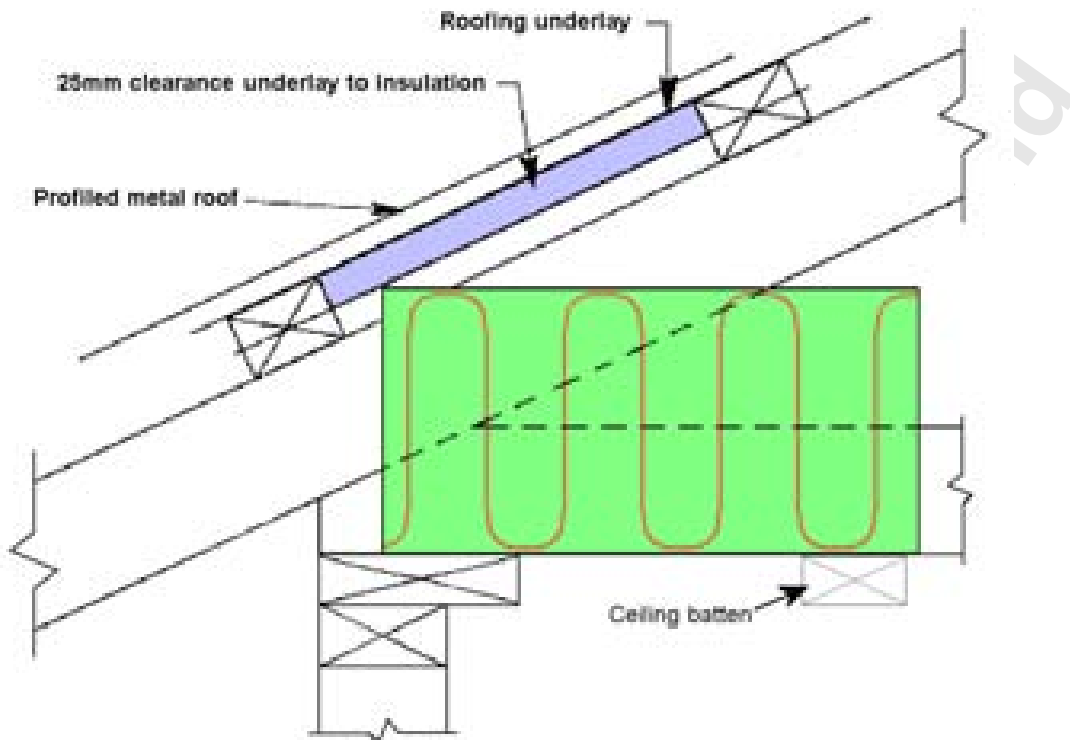
Figure 3(d) – Profiled metal roof
