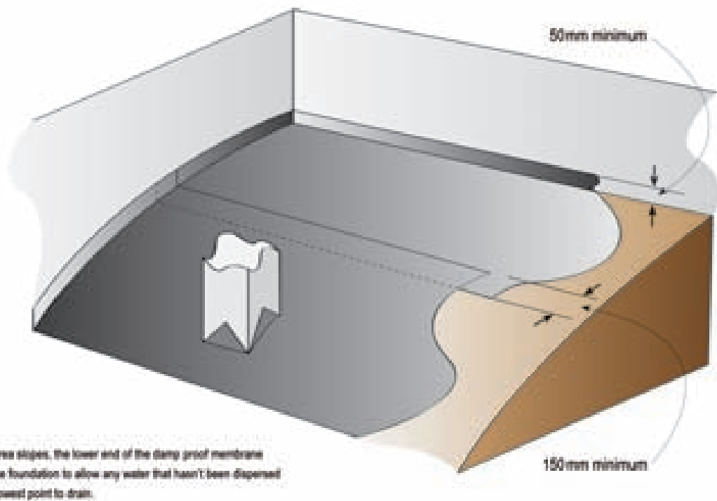
Figure 19 – On-ground vapour barrier
