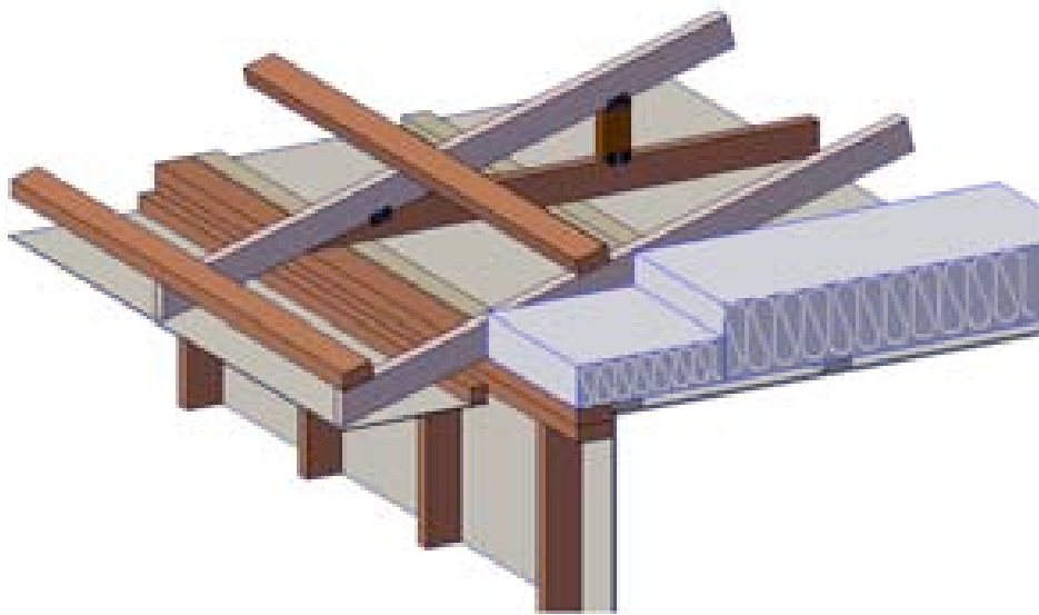
Figure 7 – Truss roof – Segment installed to top plate with full thickness blanket abutted to end of segment between truss
