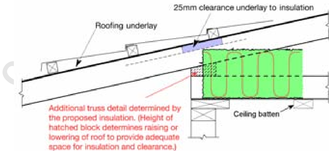
Figure 3(c) – Low pitch roof with metal tiles
