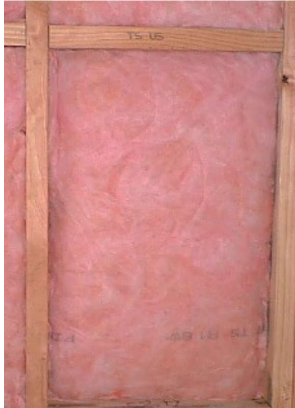
Figure 9 – Example of ‘tucking in’ showing undesirable compression of insulation at edges
