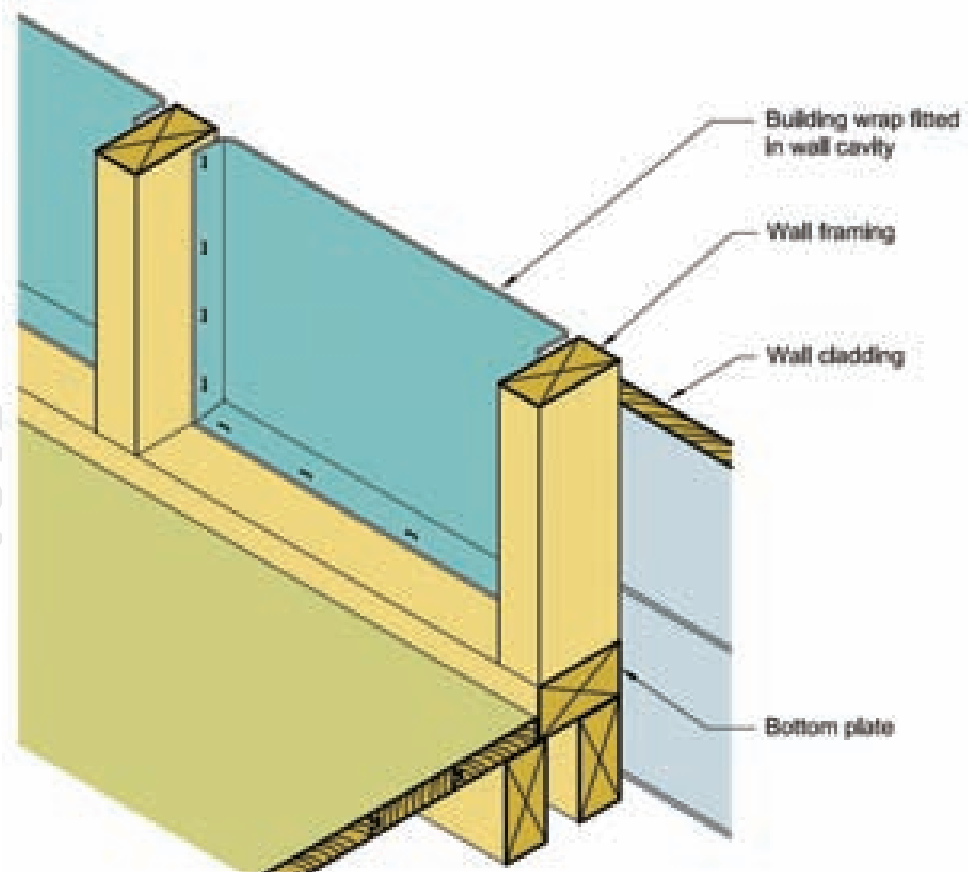
Figure 3 – Retrofitting wall underlay
